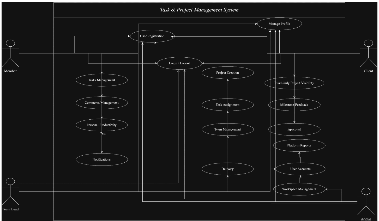
Figure: Use case diagram for the Task & Project Management System, showing the Member, Team Lead, Client, and Admin roles and their respective use cases.
